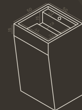
SENO RECTO INGLETADO STRAIGHT BEVELLED JOINT SINK
