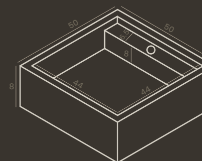
SENO RECTO INGLETADO STRAIGHT BEVELLED JOINT SINK
